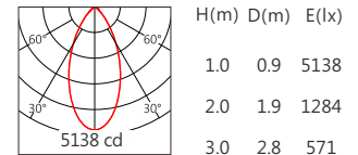
JR-5050 50° 3500K
