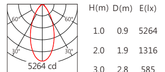
JR-5050 50° 4000K
