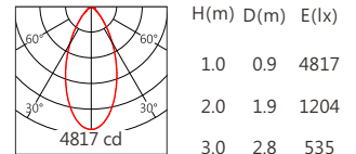
JR-5050 50° 2700K
