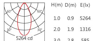
JR-5050 50° 5000K
