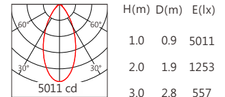
JR-5050 50° 3000K
