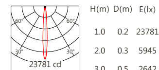
XP-E2 10° 4000K
