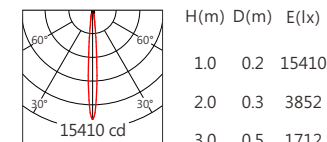
XP-E2 10° 2200K
