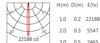
XP-E2 10° 3000K
